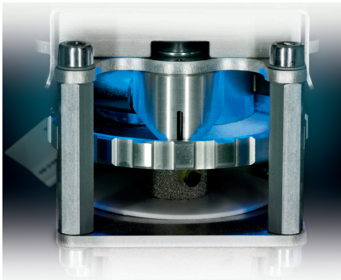
PowderMax plate dosage system
